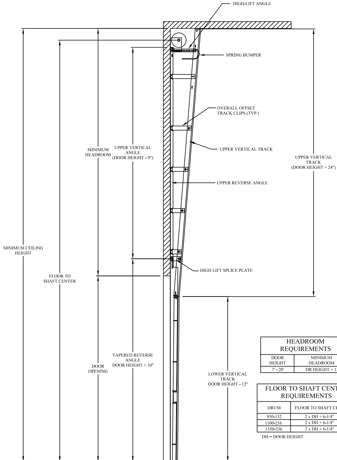
VERTICAL LIFT STANDARD 3" TAPERED REVERSE ANGLE MOUNT TRACK SET DETAIL
