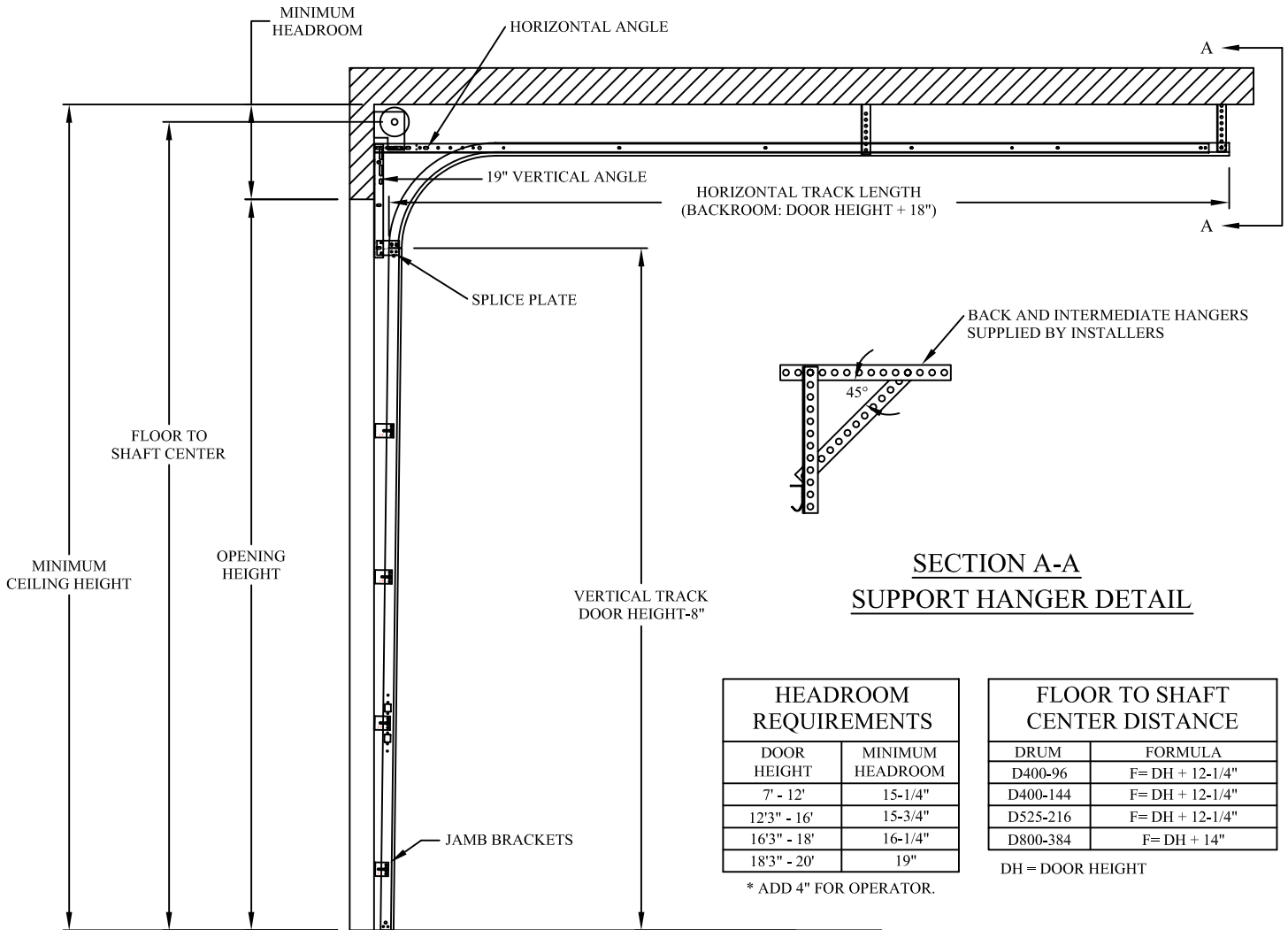
STANDARD LIFT BRACKET MOUNT TRACK SET DETAIL
