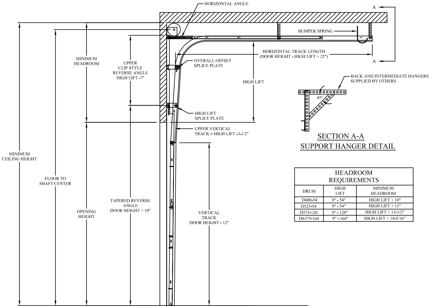
HIGH LIFT STANDARD TAPERED REVERSE ANGLE MOUNT TRACK SET DETAIL
